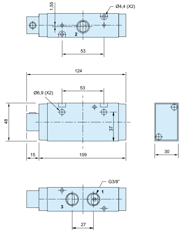
P2LCZ 3/2 Magnetventil/Feder
