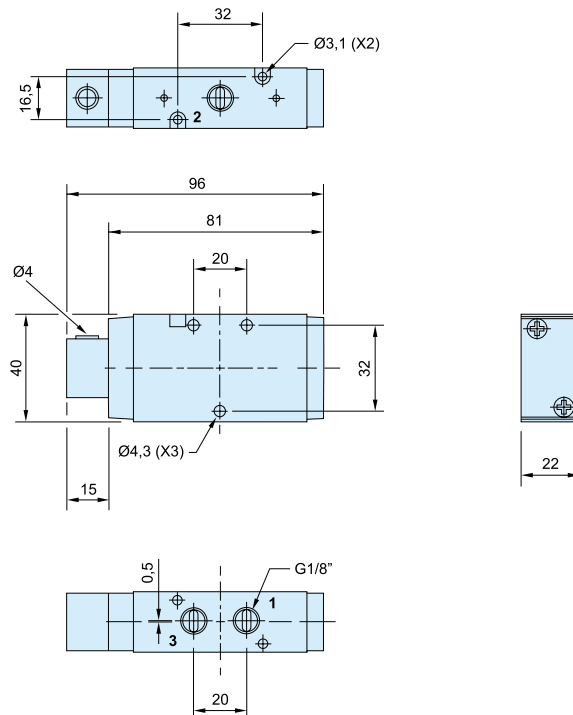
P2LAZ 3/2 Magnetventil/Feder
