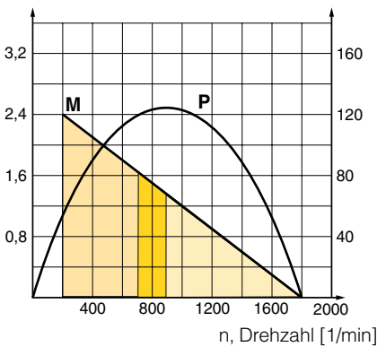
P1V-P012**1800
