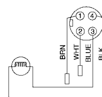
ISO 20401 4-Pin Micro (Top cover)
