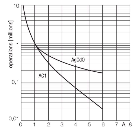
Output relay – Electrical lifetime
