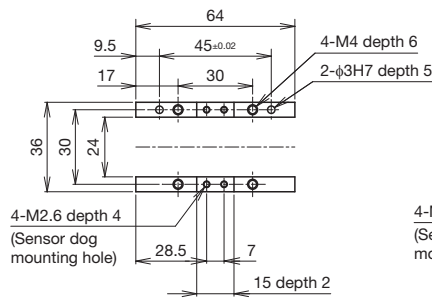
Slider (A type) details
