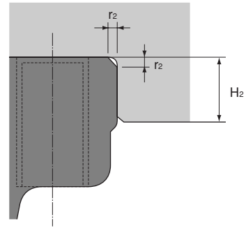
Shoulder for the LM block
