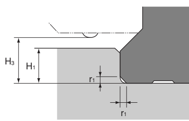
Shoulder for the LM rail
