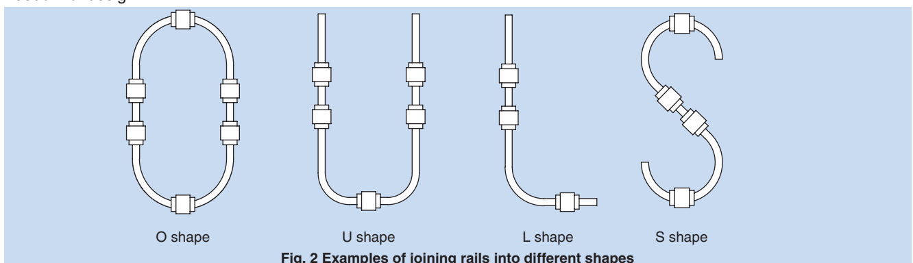
Fig. 2 Examples of joining rails into different shapes
