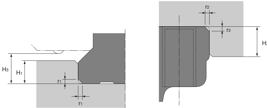
Shoulder for the LM rail
